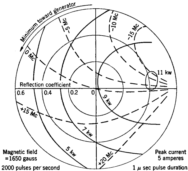
Frequency of 0 Mc contour = 3310 Mc/sec FIG. 19-12.—Rieke diagram for 2J38 and 2J39 magnetrons.
